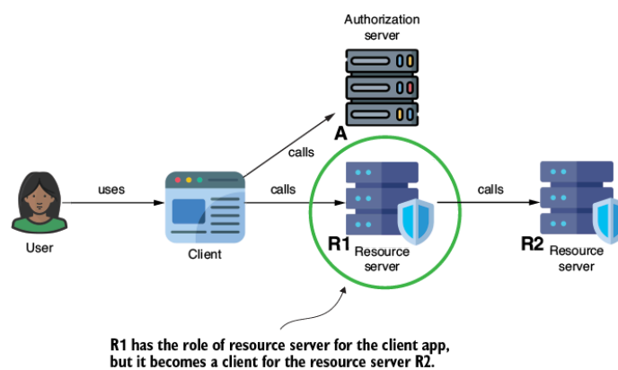
Figure 16.2 A backend app may become a client for another backend app. We discuss this case in the current chapter.
