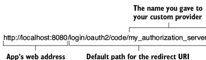
Figure 16.5 The standard redirect URI format. The last part of its path is the provider's name.
